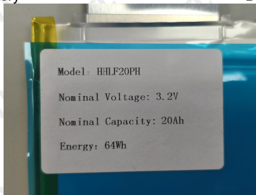
Label of battery
