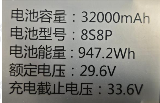
Label of battery
