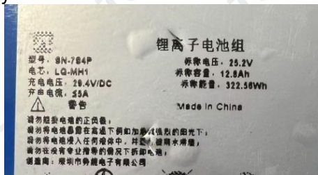
Label of battery
