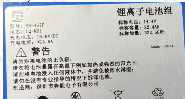
Label of battery
