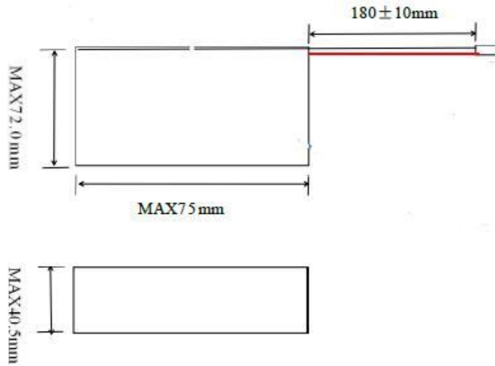
Battery
