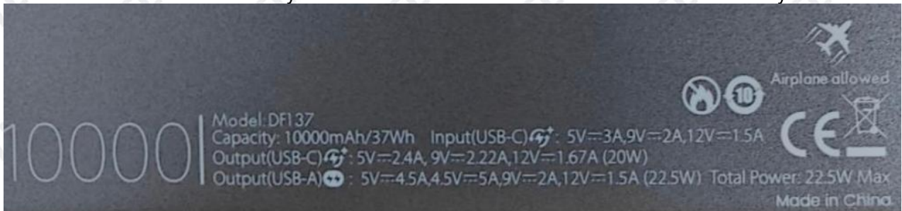
Label of battery
