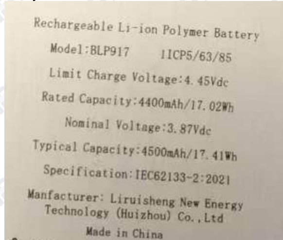
Label of battery
