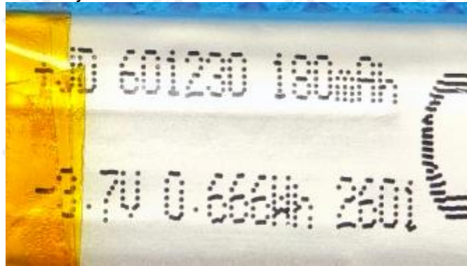
Label of battery
