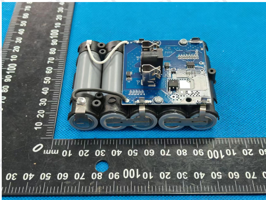
Photo 5 PCB board view
