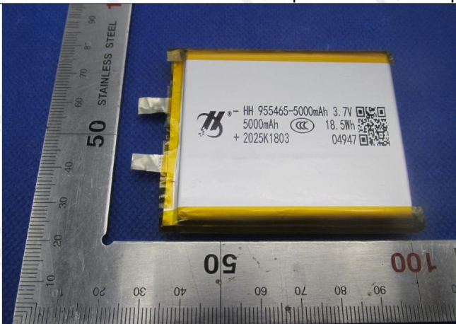
Front view of battery
