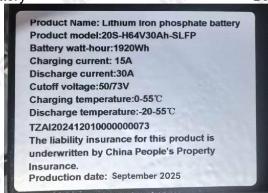
Label of battery
