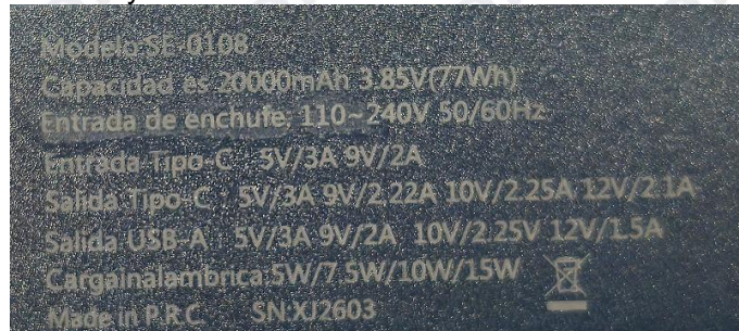
Label of battery
