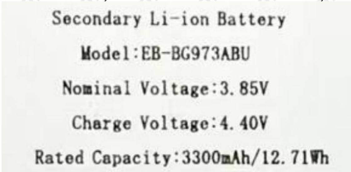
Label of battery
